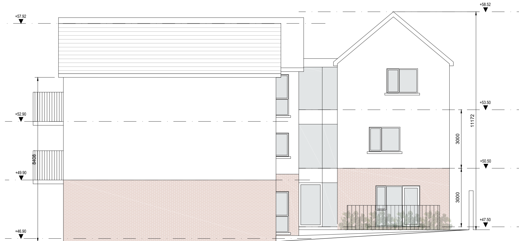
NORTHEAST ELEVATION
